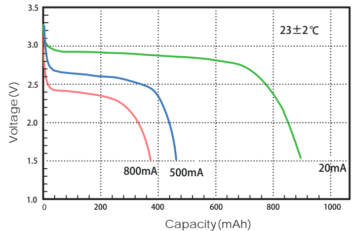
1. Typical discharge profiles at 23±2°C (at mid-discharge)
