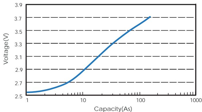
UPC1520 Capacity vs. OCV (50mA discharge at RT)
